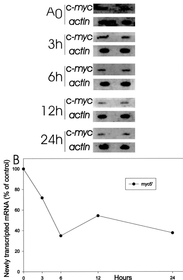
Fig. 3. Dexamethasone (Dex) suppresses transcription initiation of the c-myc gene. CEM-C7 cells were treated with 1 \mu M Dex for 0, 3, 6, 12 and 24 h and cells collected. Nuclei were isolated and nuclear run-on assays performed. A plasmid containing 148 bp of 5' flanking region and 339 bp of the first exon of c-myc or \beta - actin (control) were used as probes. Panel A: A slot blot with duplicate samples is shown. Panel B: The bands from panel A were quantified, normalized with corresponding actin bands, and data were plotted as a line graph. A representative of two independent experiments is shown.
